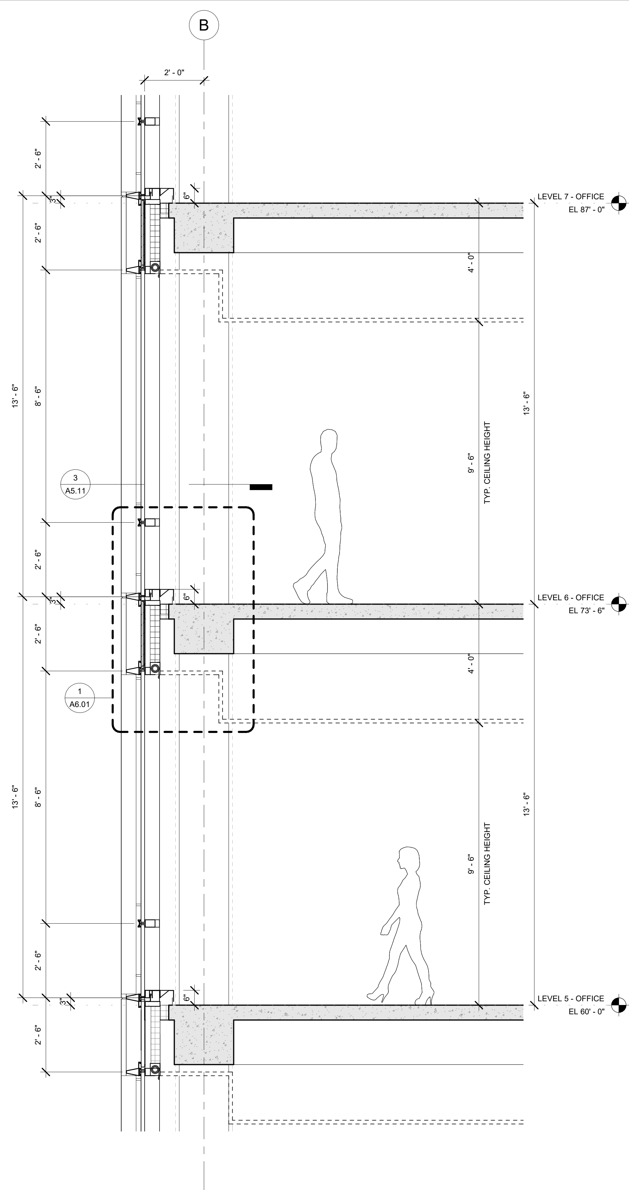
2 SECTION 1/2" = 1'-0"
